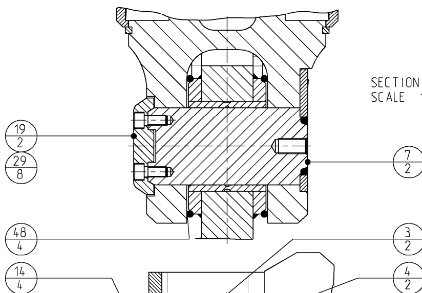
SECTION C-C SCALE 1:4
